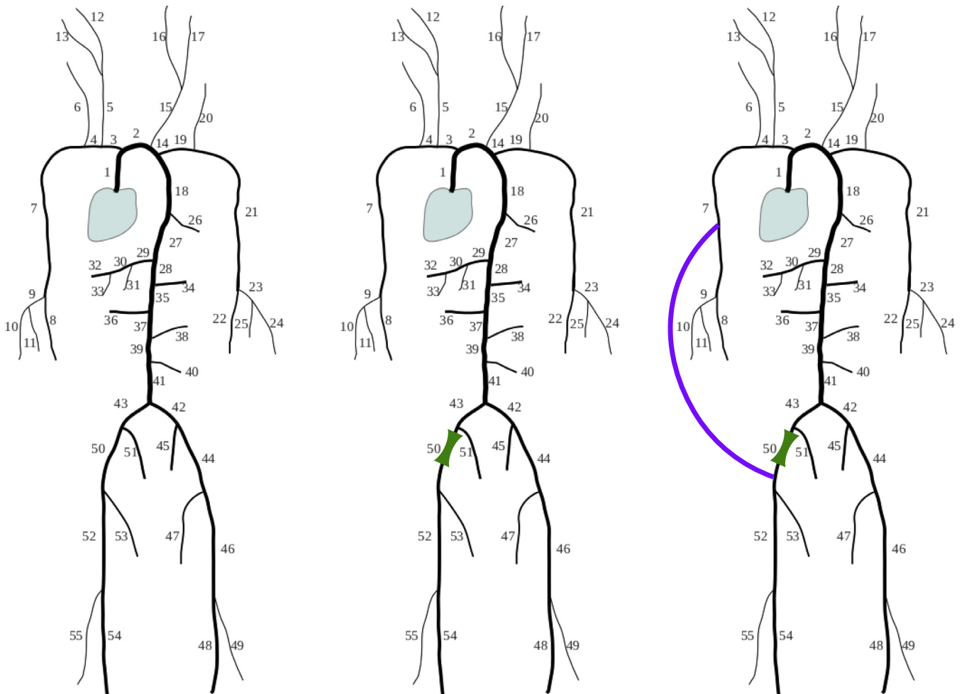
Fig. 1. Arterial tree. (a) “Healthy” network. (b) Pathological network. (c) “Repaired” network. The pathological network (b) is modeled by narrowing the cross-sectional area of the Right Iliac artery (number 50, green) and the extracorporeal bypass graft by an elastic tube (purple). In each segment, a 1D model of fluid flow with viscoelastic wall is solved numerically. The flow is imposed by given heart pulses, with a realistic reflection coefficient at the end of each terminal arteries. Table A.1 presents the geometrical and mechanical data used in numerical computations. (For interpretation of the references to color in this figure legend, the reader is referred to the web version of this article.)
