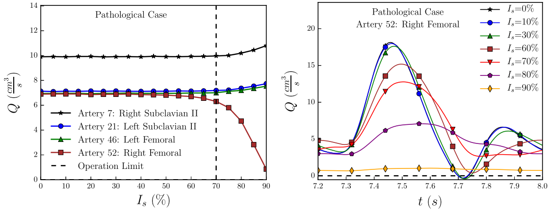
Fig. 2. (a) Flow rate averaged over a cycle as function of the obstruction degree I_s for the following arteries: Right Femoral, (number 52), Left Femoral, (number 46), Right Subclavian (number 7) and Left Subclavian, (number 21). As the ratio I_s increases, the flow rate drops in the Right Femoral artery, distal to the stenosis, whereas the flow rate increases in all other segments to compensate this drop. (b) Instantaneous flow rate as function of time over a cycle in the Right Femoral artery (number 52) for different degree of obstruction. As the ratio I_s increases, the waveform loses its pulsatility and flattens and the average flow rate drops.
