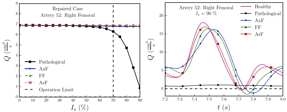
Fig. 4. (a) Averaged flow rate over a cycle as function of the degree of obstruction I_s (Artery 52: Right Femoral) (b) instantaneous flow rate as function of time over a cycle (Artery 52: Right Femoral) for healthy, pathological with I_s = 90\% and for the three bypasses. We observe that for all three bypass graft configurations, we are able to recover the target healthy flow rate (average values and waveform) distal to the stenosis.
