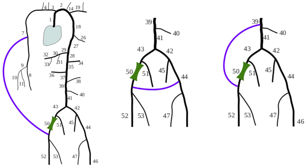
Fig. 3. Sketch of three bypasses with the donor artery: (left) Axillo-Femoral (AxF) and donor artery, Right Axillary artery (number 7), (center) cross-over-Femoral (FF) and donor artery, Left Femoral artery (number 44) and (right) Aorto-Femoral (ArF) and donor artery, Abdominal Aorta (number 39).
