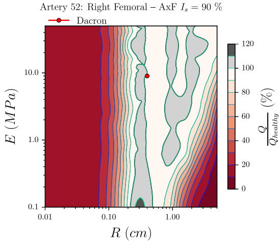
Fig. 8. Contour plot for the normalized time-averaged flow rate \frac{Q}{Q_{healthy}} as function of the Young modulus E and the radius R for a stenosis of I_s = 90\% . The red circle corresponds to the actual values of the Young modulus E and the radius R used in numerical simulations, which are situated in an optimal zone (100%). When the radius decreases, the resistance of the tube increases and therefore less flow is bypassing through the bypass graft. When Young's modulus decreases, the tube becomes more compliant and stores more flow. Both behaviors reduce the quality of the bypass graft. (For interpretation of the references to color in this figure legend, the reader is referred to the web version of this article.)
