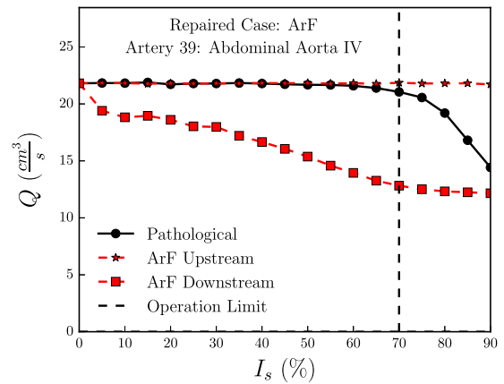
Fig. 6. Aorto-Femoral bypass graft: average flow rate over a cycle at the donor artery (Artery 39). Upstream of the proximal anastomosis, the flow rate remains unchanged since blood flow passing through the bypass graft to vascularize the right leg was already supplied by the Aorta in the healthy case. Downstream of the proximal anastomosis, the flow rate decreases with the degree of obstruction I_s since now only the blood supplying the left leg is passing downstream of the proximal anastomosis.
