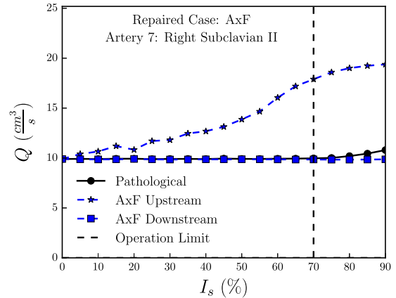
Fig. 7. Axillo-Femoral bypass graft: averaged flow rate over a cycle at the donor artery (number 7). Upstream of the proximal anastomosis, the flow rate increases to properly vascularize the bypass graft, depending on the degree of obstruction I_s . Downstream of the proximal anastomosis, we recover the healthy ( I_s = 0\% ) flow rate.
