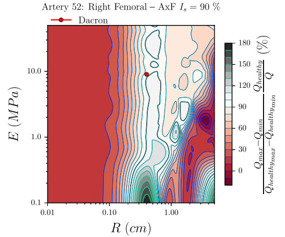
Fig. 9. Contour plot for the normalized peak to peak flow rate \frac{Q_{max} - Q_{min}}{Q_{max} - Q_{min}} \frac{Q_{healthy}}{Q} as function of the Young modulus E and the radius R for a stenosis of 90%. The red circle corresponds to the actual values of the Young modulus E and the radius R used in numerical simulations. (For interpretation of the references to color in this figure legend, the reader is referred to the web version of this article.)
