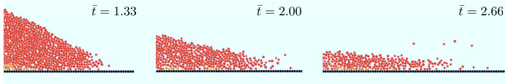
FIGURE 18. Snapshots of the flow front at \bar{t} = 1.33 , \bar{t} = 2.00 and \bar{t} = 2.66 for a discrete numerical simulation with aspect ratio a = 6.26 . Note the rough plane obtained by "gluing" grains.
