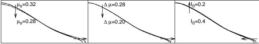
FIGURE 16. A collapse at time \bar{t} = t/(H_0/g)^{1/2} = 2 with aspect ratio a = 1.42 , with \mu_s = 0.32 , I_0 = 0.4 and \Delta\mu = 0.28 in the three panels. In each panel, a second computation with only one parameter changed is displayed. Left, \mu_s is decreased: \Delta\mu , and I_0 preserved. Center, case with a smaller \Delta\mu , but same I_0 = 0.4 and \mu_s = 0.32 , Right, case with a smaller I_0 , but same \Delta\mu = 0.28 and \mu_s = 0.32 .
