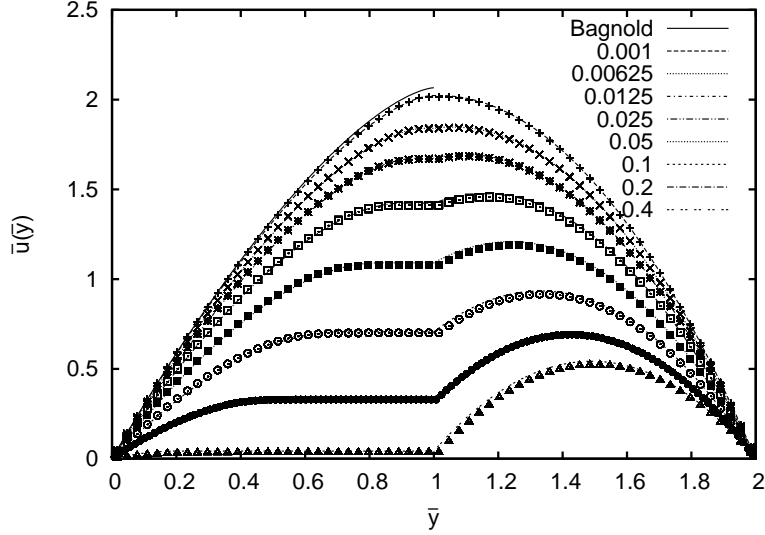
FIGURE 5. Comparisons of the Gerris numerical solution (symbols) and the solution of the system of ODEs (2.18) corresponding to the case of two layers, solution (lines) for the two (phase) layer problem, for \nu_f/(\sqrt{gH^3}) = 0.1 and different values of the density ratio \rho_f/\rho from 0.001 to 0.4 (large values have no physical application but validate the numerics). The slope is \alpha = 0.43 . The corresponding Bagnold profile is plotted with a solid line for 0 < \bar{y} < 1 .
