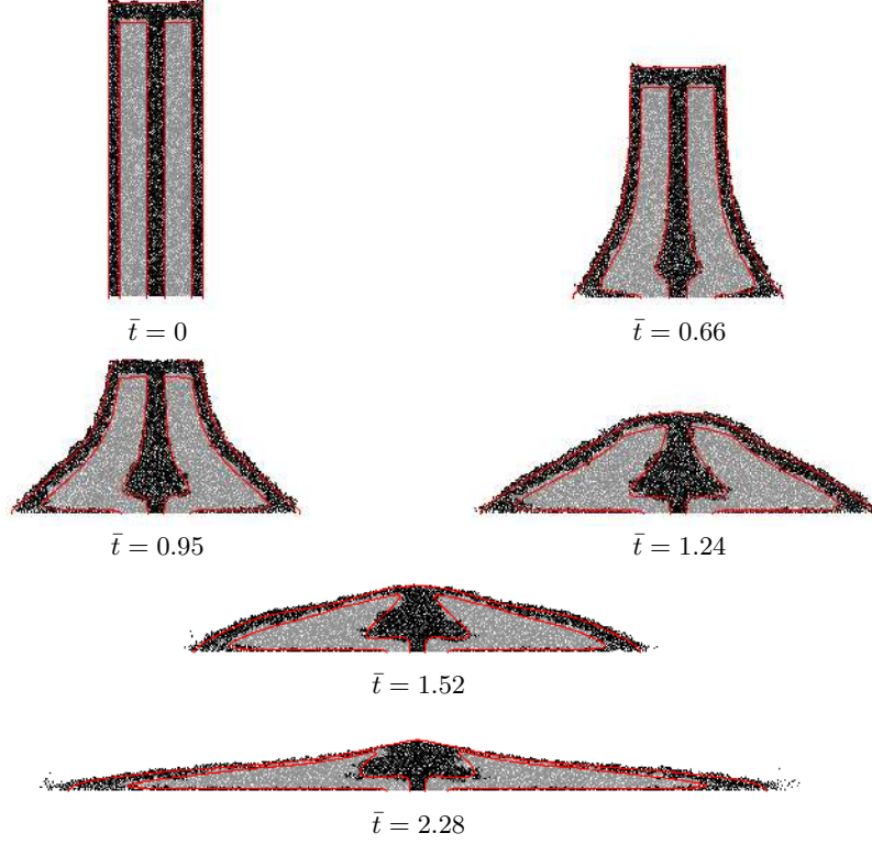
FIGURE 10. Comparison between the \mu(I) continuum model (red line) and contact dynamics simulations (grains) for an aspect ratio a = 6.26 at different times (non-dimensionalized by \sqrt{H_0/g} ). The parameters of the \mu(I) -rheology are \mu_s = 0.32 , \Delta\mu = 0.28 and I_0 = 0.4 (color online).
