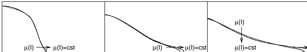
FIGURE 15. A collapse at time t/(H_0/g)^{1/2} = 1, 2 and 3 , with aspect ratio a = 1.42 , with \mu_s = 0.32 , I_0 = 0.4 and \Delta\mu = 0.28 in the three panels. In each panel, the same case with a constant \mu(I) = 0.33 (cst) is plotted, the arrow is from the variable \mu(I) to the constant \mu(I) = 0.33 .
