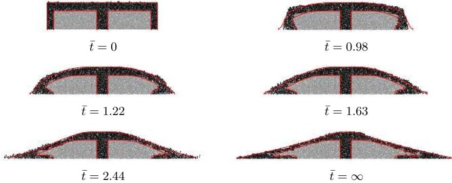
FIGURE 8. Comparison between the \mu(I) continuum model (red line) and contact dynamics simulations (grains) for an aspect ratio a = 0.5 at different times (non-dimensionalized by \sqrt{H_0/g} ). The grains are colored in the initial heap, which allows one to track the displacement, see (Staron & Hinch 2005). The parameters of the \mu(I) -rheology are \mu_s = 0.32 , \Delta\mu = 0.28 and I_0 = 0.4 . (color online).
