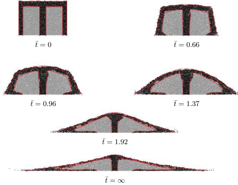
FIGURE 9. Comparison between the \mu(I) continuum model (red line) and contact dynamics simulations (grains) for an aspect ratio a = 1.42 at different times (non-dimensionalized by \sqrt{H_0/g} ). The parameters of the \mu(I) -rheology are \mu_s = 0.32 , \Delta\mu = 0.28 and I_0 = 0.4 (color online).
