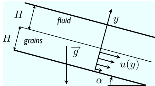
FIGURE 1. Sketch of the granular material moving along a flat rigid bed inclined at an angle \alpha ; the coordinate x is along the slope, y is the coordinate normal to the plane. The bottom is at y = 0 , and the top is at y = 2H . The thickness of the flow is H (much larger than the grain size d \ll H ). The flow is parallel to the slope u = u(y) and v = 0 . In section 2.3.3 the granular medium is covered by a fluid, and there is an interface at y = H and a rigid wall at y = 2H , thus forming a channel.
