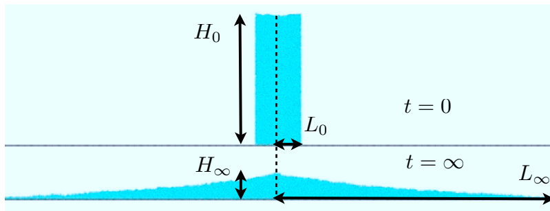
FIGURE 6. Schematic illustration of the column collapse experiment in two dimensions. The initial height of the column is H_0 , its initial half-width is L_0 and a = H_0/L_0 is the aspect ratio; the final maximum thickness is H_\infty and the final half-width, or run-out, is L_\infty .
