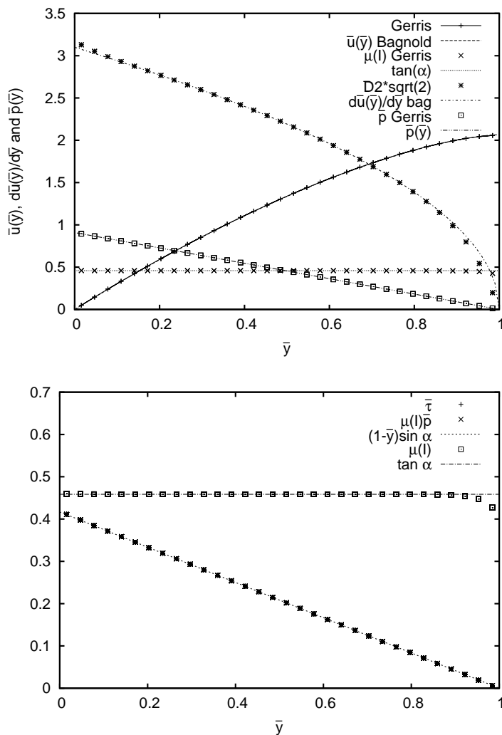
FIGURE 2. Comparison between (a) analytical and (b) computed (on a 32 \times 32 grid) profiles for a single granular layer ( 0 < \bar{y} < 1 ) with the \mu(I) -rheology. The slope angle is \alpha = 0.43 , and \bar{d} = 1/25 . (a) analytical (2.16) and Gerris solution for the pressure, velocity and velocity gradient. (b) Comparison of shear stress \bar{\tau} = \bar{\eta} d\bar{u}/d\bar{y} (+), \mu(I)\bar{p} (x) and exact solution (dashed line); and comparison of the computed \mu(I) ( \square ) with the exact solution \tan\alpha (dot-dashed line).
