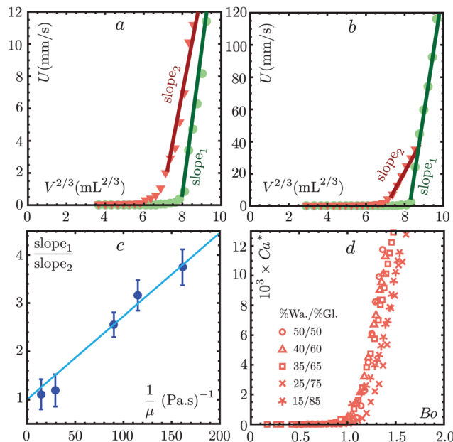
Fig. 7 (a) Droplet speed in the first (green circles) and second (red triangles) regimes in the case of a 75% glycerol–25% water mixture, as a function of V^{2/3} , where V is the droplet volume. The linear part of the curve is fitted and the slope of the fit is denoted \text{slope}_1 for the first regime and \text{slope}_2 for the second regime. (b) Same graphic for a 50% glycerol–50% water mixture. (c) Ratio between the slopes measured for the linear part in the first and second regimes, as a function of the inverse of the water–glycerol mixture viscosity. An affine relationship with intercept equal to unity is found, in agreement with our simple model. (d) A modified Capillary number Ca^* is used to plot the speed of the droplets in the second regime as a function of their weight, through the Bo number.
