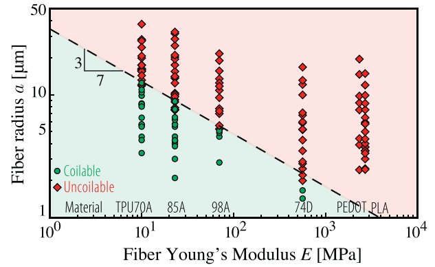
Fig. 5. Theoretical and experimental coilaible and uncoilaible fibers of different materials in the corresponding optimal silicone oil droplet. The theoretical limit between the coilaible and uncoilaible systems is given in Eq. (10) and experiments validate the theoretical power law a_{max} \propto E^{-3/7} and the corresponding prefactor. For PEDOT:PSS and PLA fibers, no coiling ever occurred as we were not able to produce thin enough fibers. \gamma = 21 mN/m, \rho g = 9600 N/m 3 .
