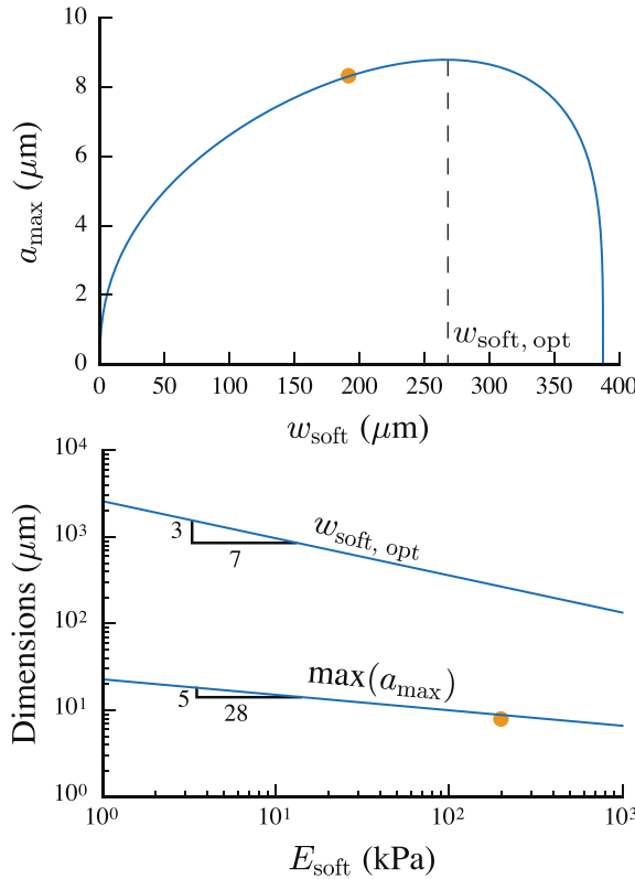
Fig. 9. Optimal dimensions for the fiber and the auxiliary beam width. The auxiliary beam has Young's modulus E_{\text{soft}} (PVS) and an aspect ratio k = h_{\text{soft}}/w_{\text{soft}} = 0.34 (value used experimentally). The silicone oil drop has \gamma = 21 mN/m and \rho g = 9600 N/m ^3 . The core fiber in this example has a Young's modulus of E = 1 GPa. Top: Largest coiled fiber radius a_{\text{max}} as a function of the width w_{\text{soft}} of the auxiliary beam of Young's modulus E_{\text{soft}} = 200 kPa as given by Eq. (13). The function has a maximum at w_{\text{soft}} = w_{\text{soft, opt}} , see Eq. (14). The orange dot corresponds to the experimentally-used auxiliary beam, which was not far from being optimal. Bottom: w_{\text{soft, opt}} as a function of the Young's modulus E_{\text{soft}} of the auxiliary beam, Eq. (14), and the corresponding maximum coiled core fiber's radius \max(a_{\text{max}}) , Eq. (15). The orange dot shows the value a_{\text{max}} , given by Eq. (13), for the experimentally used auxiliary beam.
