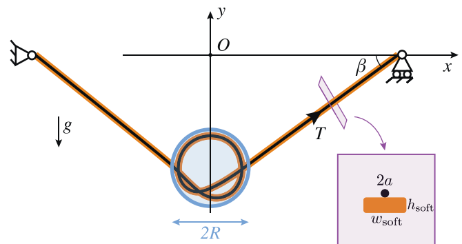
Fig. 6. Cylindrical fiber of radius a affixed to a soft beam (rectangular cross section: height h_{soft} , width w_{soft} ) undergoing coiling inside a liquid drop of radius R in the gravity field. Due to gravity, the coiled state is sagging and the equilibrium state displays a sagging angle \beta which depends on the system physical parameters. The composite fiber (core fiber + soft beam) inherits the large beam's perimeter but its bending stiffness mainly depends on that of the core fiber.
