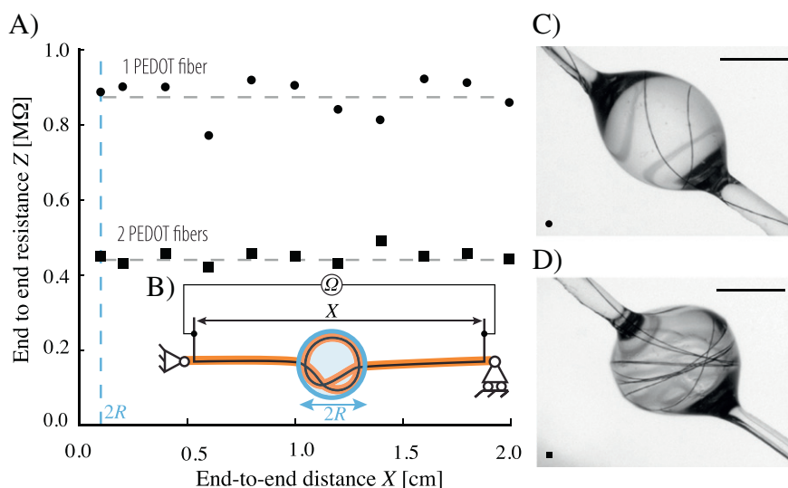
Fig. 10. Coiling conductive micronic PEDOT:PSS fibers ( a_{\text{PEDOT}} = 4.2 \mu m ) inside a silicone oil droplet with the assistance of a soft auxiliary beam. This composite fiber conducts electricity throughout the 1900% stretching test. (A) Electrical resistance versus end-to-end distance X of the fiber for 1 and 2 PEDOT:PSS fibers and one soft auxiliary PVS beam. The resistance was measured between two points, further apart than the actual ends of the auxiliary beam (total fiber length: 3.5 cm), see (B). Pictures (C) and (D) show macroscopic snapshots of the droplets for X = 1.6 cm and X = 0.8 cm for 1 and 2 PEDOT:PSS fibers respectively. The dark PEDOT:PSS can easily be spotted inside and outside the droplet. The PVS beam, however, is only visible outside the droplet due to a refraction index too close from that of the silicone oil. Scale bar on both pictures: 500 \mu m .
