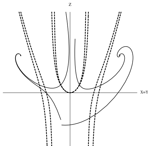
FIG. I-21 – Critical points separated by semipermeable surfaces of type (I.5-18) in case \alpha . The far left (resp. right) zone is a part of the bassin of attraction of C^- (resp. C^+ ).
