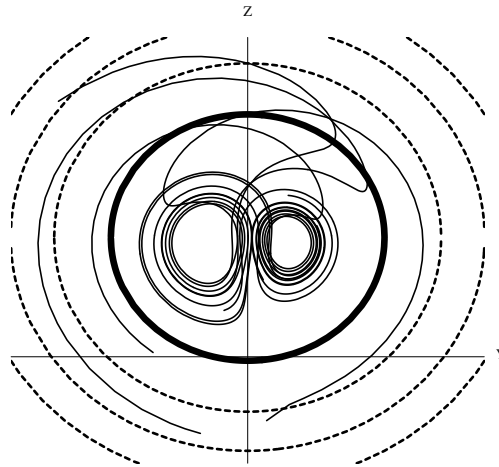
FIG. I-16 – Chaotic attractor stuck inside semipermeable cylinders of radius \frac{1}{a_1} . The bolded circle corresponds to the smallest cylinder.
