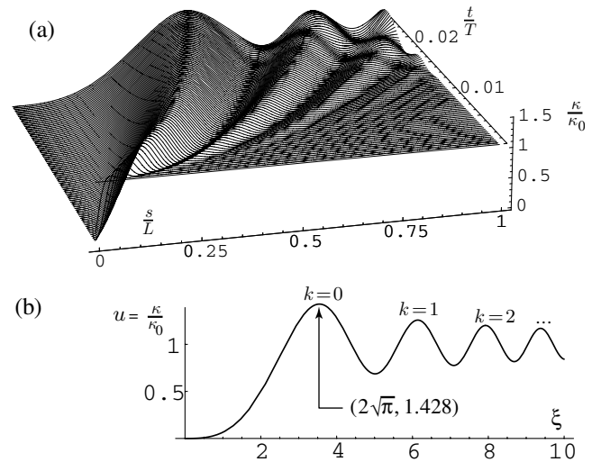
FIG. 2. (a) Numerical solution of the Kirchhoff Eq. (1) with clamped-free boundary conditions, for a uniform initial curvature \kappa_0 . The curvature at the free end \kappa(0, t) relaxes to zero within the first few time steps (quick relaxation of the incompatible curvature near free end) while it is given in the intermediate regime (2) by the universal self-similar solution (4), shown in (b) as a function of \xi = s/\sqrt{\gamma t} . At later times, for t \sim T , reflections are generated from the clamped end s = L .
