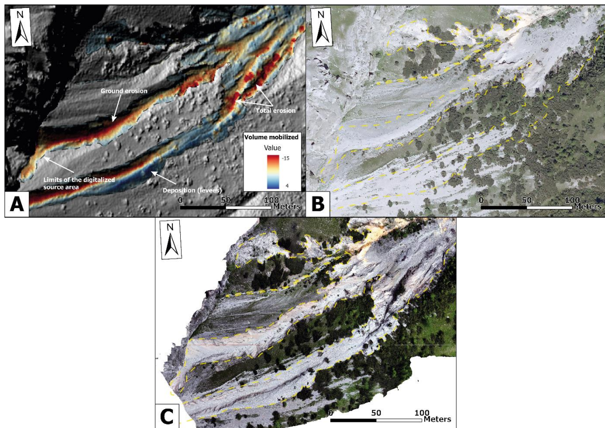
Fig.4 : Illustration of altimetric differences at the head of the Rabay valley gullies ( DTM_{2021} - DSM_{2020} ) across different temporal scales: A) DSM_{2021} post-flood B) orthoimages from July 2020 (pre-flood) C) orthoimages from October 5 to 7, 2020 post-flood. A) Overlaid with the outcome of equation (1), delineating erosion zones (in red) and deposition zones (in blue). The delineated working area is marked by the dashed yellow line. In these visuals, we can observe areas with sparse vegetation where DSM_{2020} equals DTM_{2021} , allowing for direct estimation of ground erosion . Total erosion is notably pronounced in certain areas, reaching maximum values of up to -15m.
