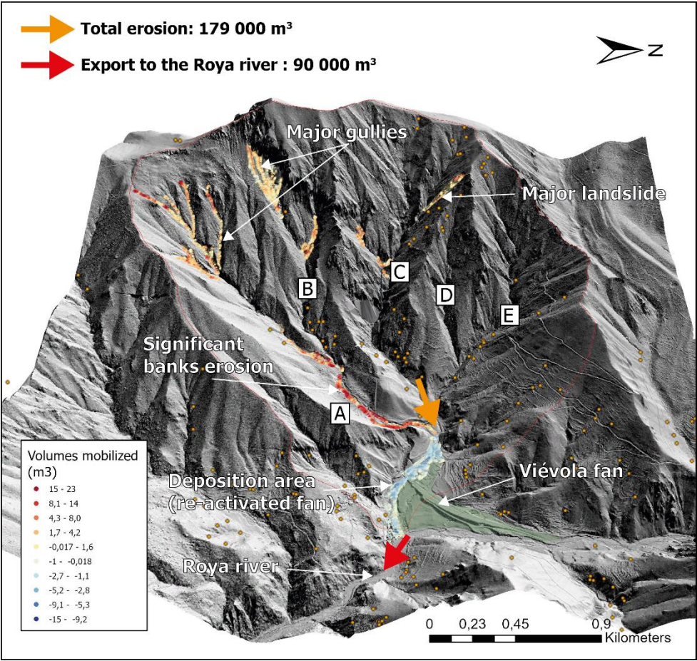
Fig. 5 : Spatial representation of mobilized volumes in the Viévol watershed, including calculated erosion and deposition areas based on the methodology outlined above. The geomorphological map (Figure 2) provides a plan view of the study area. A) corresponds to the Dente torrent, B) the Rabay torrent, C) the Morte torrent, D) the Para torrent, and E) the Scabrie torrent. Thin red line represent Viévol catchment. The orange dots represent landslides that occurred during the event. The green polygon represents the surface area of the Viévol fan, estimated to be 250,000 m² using ArcGIS Pro. Erosion areas are indicated by yellow to red dots, with their surfaces detailed in Table 3. Blue dots correspond to deposition on the Viévol fan, with an estimated surface area of 67,036 m².
