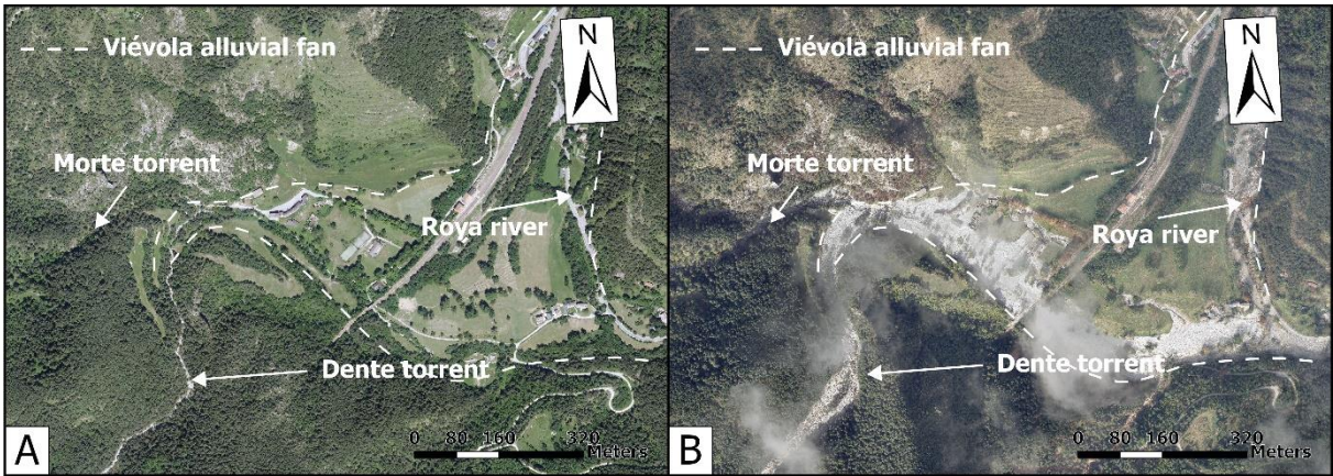
Fig. 2 : The Viévola resort camp is depicted in two snapshots, showcasing the conditions before and after the October 2020 flood. In the post-flood image, the torrents and the Roya River on the right side of the picture exhibit significant changes, with noticeable increases in depth and width. The southern part of the Viévola alluvial fan was heavily embanked following the flood.
