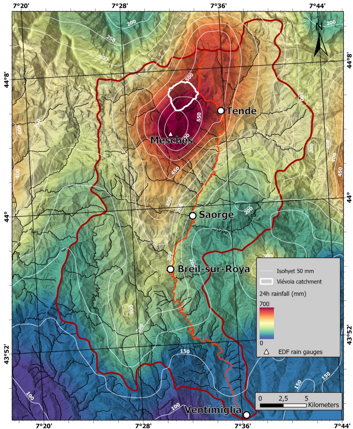
Fig.1 : 24 hr rainfall map in the Roya valley, as modified by Liébault et al. (2024). The catchment divide is highlighted in red, stream networks are depicted as thin black lines, and the Roya River is represented by a thick dark orange line. The Viévola catchment area is delineated in the upper part of the valley in light white.
