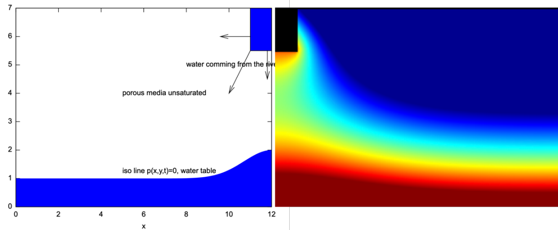
FIGURE 24 – Vauclin’s experiment, and a numerical plot with Basilisk
