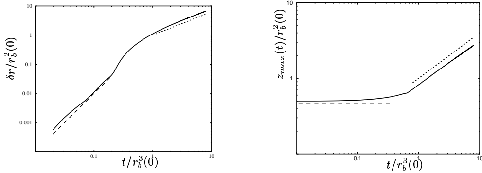
FIGURE 6. Two quantities characterizing retraction, \delta r = r_b(t) - r_b(0) and z_{max} as functions of time in rescaled units. Long-dashed and dotted lines represent power-law approximations to the early and long-time behavior, respectively. We find \delta r \propto t^2 for early times, while z_{max} remains constant. For late times \delta r \propto t^{0.8} and z_{max} \propto t^{0.6} ; both behaviors are in agreement with (5.2).
