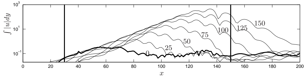
FIGURE 5. Snapshots of y -integrated streamwise velocity at times 0, 25, \dots , 150, showing propagation of wavepacket in the eigenmode system. The thick line shows the initial disturbance. The vertical lines indicates the approximate start and end of the recirculation region.
