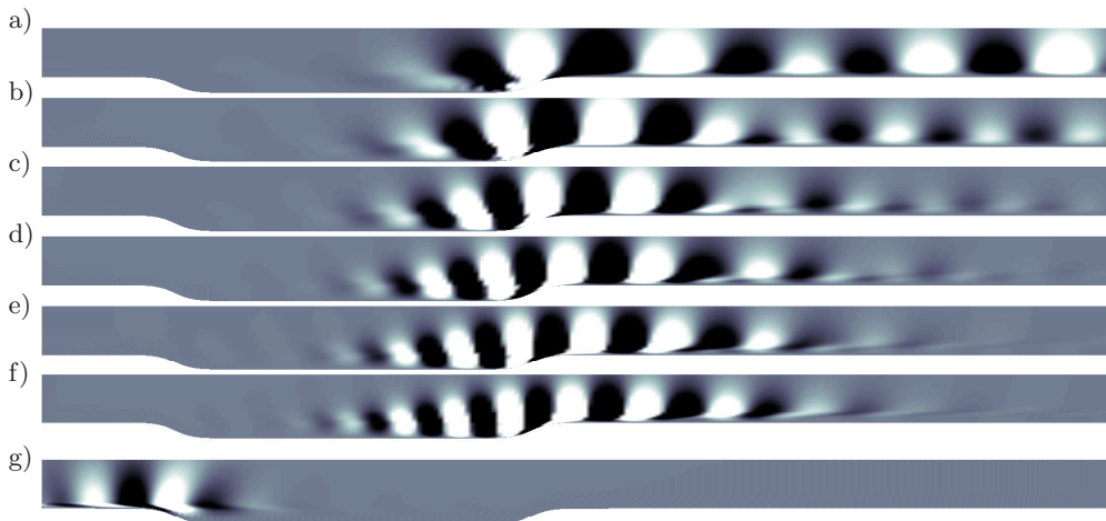
FIGURE 3. a)-f) Vertical velocity components of direct eigenfunctions corresponding to the eigenvalues labelled m_1 - m_6 in figure 2, respectively. g) Adjoint eigenfunction corresponding to m_3 , the most unstable eigenvalue. Black indicates large negative values and white indicates large positive values, with the grey tones adjusting accordingly. The domain is truncated at y = 14 .
