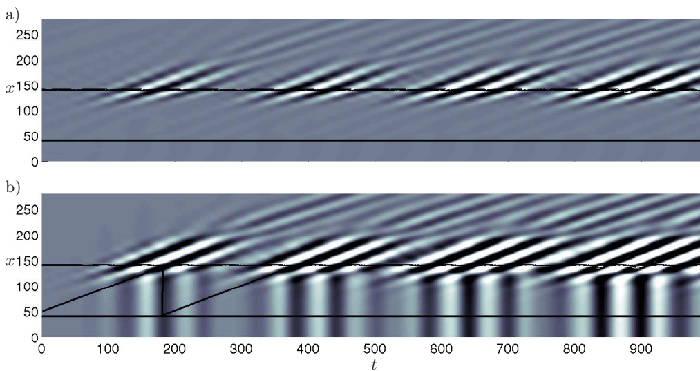
FIGURE 6. x/t diagram for a) the vertical flow velocity at y = 2 and b) the pressure at y = 10 , tracing the quantities in the streamwise direction and in time at their respective vertical position. Black indicates large negative values whereas white indicates large positive values. The flow initial condition is the optimal initial condition. The horizontal lines show the location of the cavity lips. The oblique lines trace the path of the wavepacket back to its origin and the triggering position at the upstream lip of the cavity at the first reflection.
