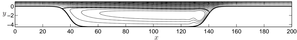
FIGURE 1. Streamlines of steady state base flow solution used for stability analysis at Re = 350 . The thick line represents the zero level contour. Note the large aspect ratio of L/D \approx 25 and the smooth lips.
