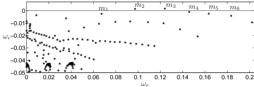
FIGURE 2. Eigenvalues of the direct problem (2.4). There are two unstable modes. The modes labelled m_1 - m_6 is depicted in figure 3.
