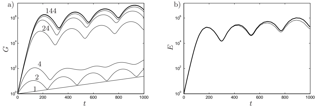
FIGURE 4. a) Envelope of maximum energy growth from initial conditions. The different lines correspond to increasing number of eigenmodes included in the optimization, 1, 2, 4, 24, . . . , 124, 144 from bottom to top. b) One realization using initial condition based on 100 modes, thick line shows eigenmode system integrated in time and thin line shows DNS evolution.
